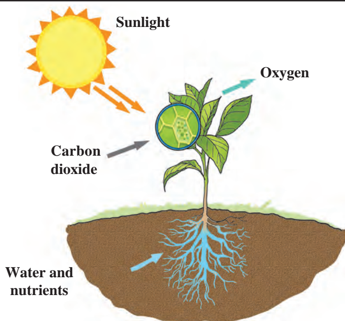
2.5 : Photosynthesis
